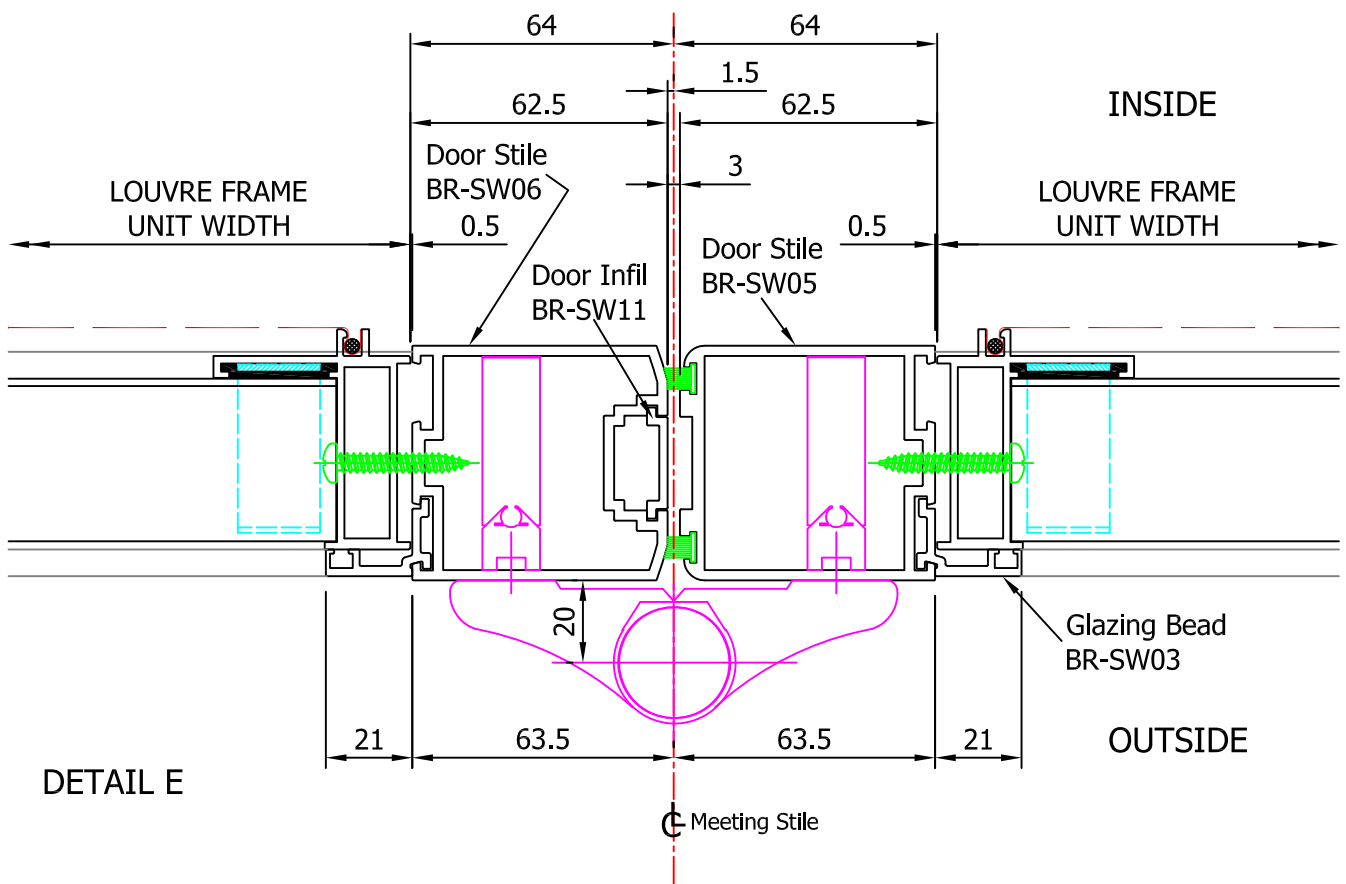
4 LEAF BI-FOLDING DOOR MEETING STILE HINGE DETAIL
